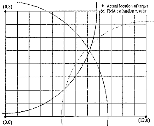
Figure 9. TMA localization of tag at (7, 5)
