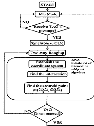
Figure 5. Flow chart of TMA scheme
