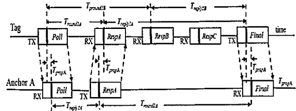
Figure 3. Multiple station DS-TWR scheme
