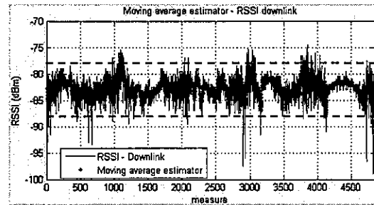
Figure 5. Downlink RSSI – Moving Average Estimate.
