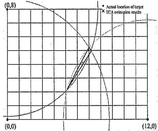
Figure 8. TCA localization of tag at (7, 5)
