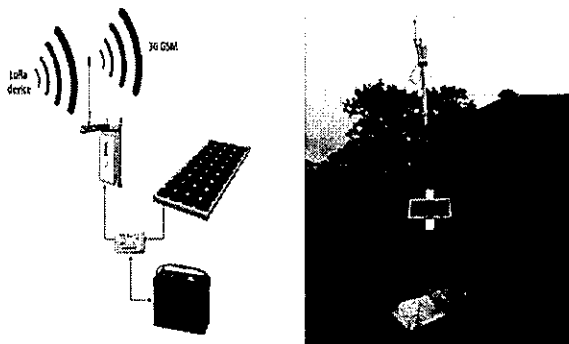
Figure 6 : autonomous LoRa antenna system
