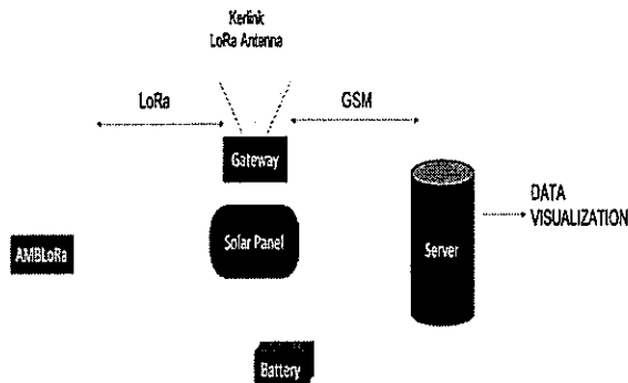
Figure 3 : Sytem architecture
