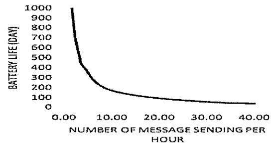
Figure 11 : Battery Lifetime of AMBLoRa
