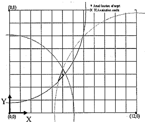
Figure 7. TCA localization of tag at (5, 3)
