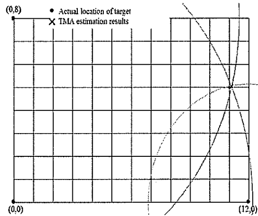
Figure 10. TMA localization of tag at (11, 5)
