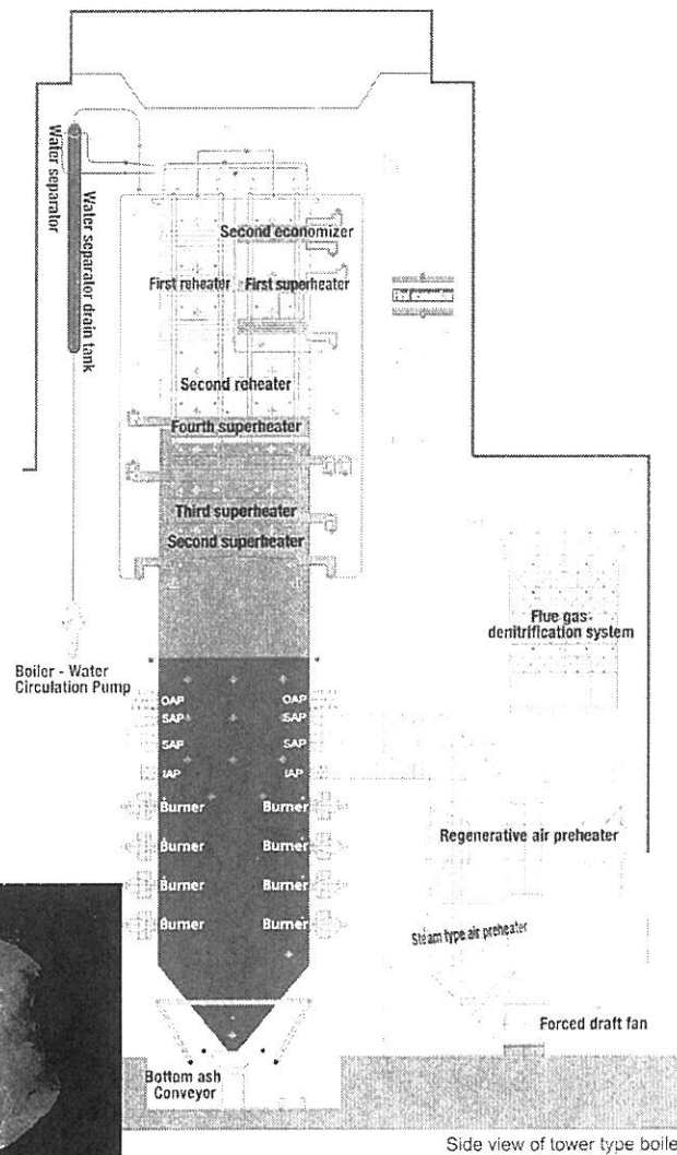
Side view of tower type boiler
