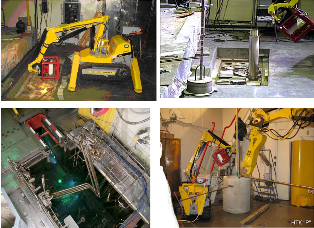
Fig. 2. Radiation survey of SNF repository and the removal of spent fuel from it and from the reactor pool.
