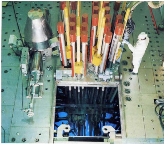
Fig. 2. MR reactor: left - view from above; right – plan and horizontal cross-section of reactor pool and storage pool (1 – reactor pool; 2 – storage pool; 3 – lock gate; 4 – shielding slabs over loop channel connections with the loop; 5 – gamma irradiator tube plate; 6 – gamma irradiator chamber; 7 – FA channel retrieved from reactor; 8 – tank containing equipment for underwater cutting of channels of any type; 9 – loop FA channel retrieved from reactor).
