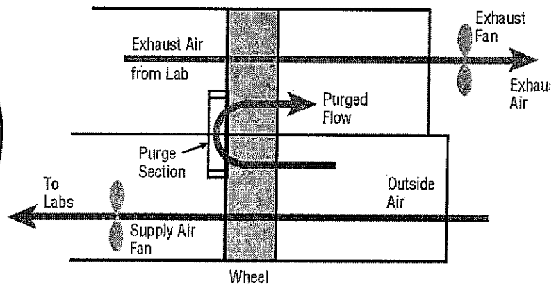
Side Cross Section with Purge Section
