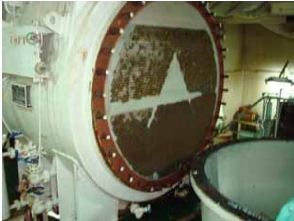
Condenser for T/G
