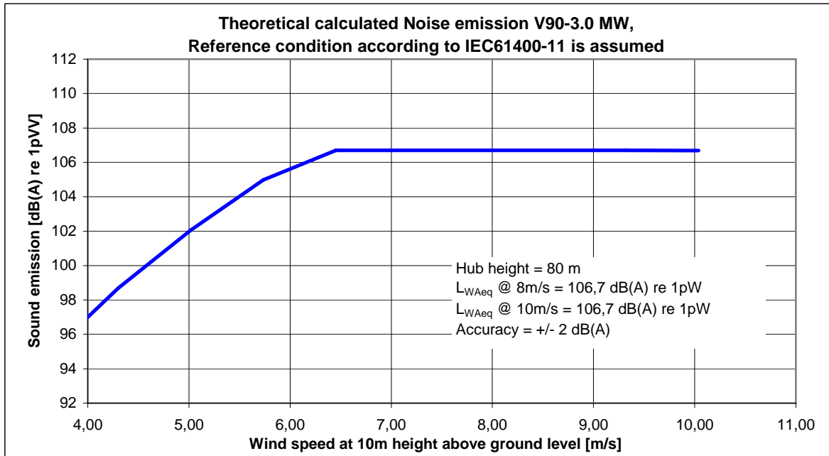
Fig. 9 Noise Emission V90 – 3.0 MW, 60 Hz: Mode 2 measures at 8 m/s in 10 m height
