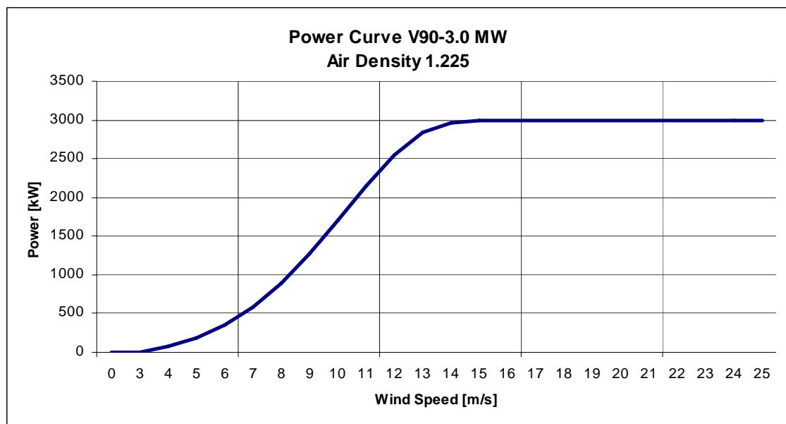
Fig. 3 Power curve for VESTAS V90 – 3.0 MW, 60 Hz, Mode 1
