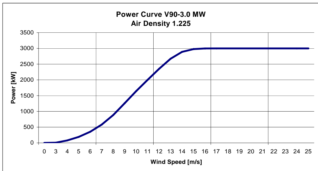
Fig. 4 Power curve for VESTAS V90 – 3.0 MW, 60 Hz, Mode 2
