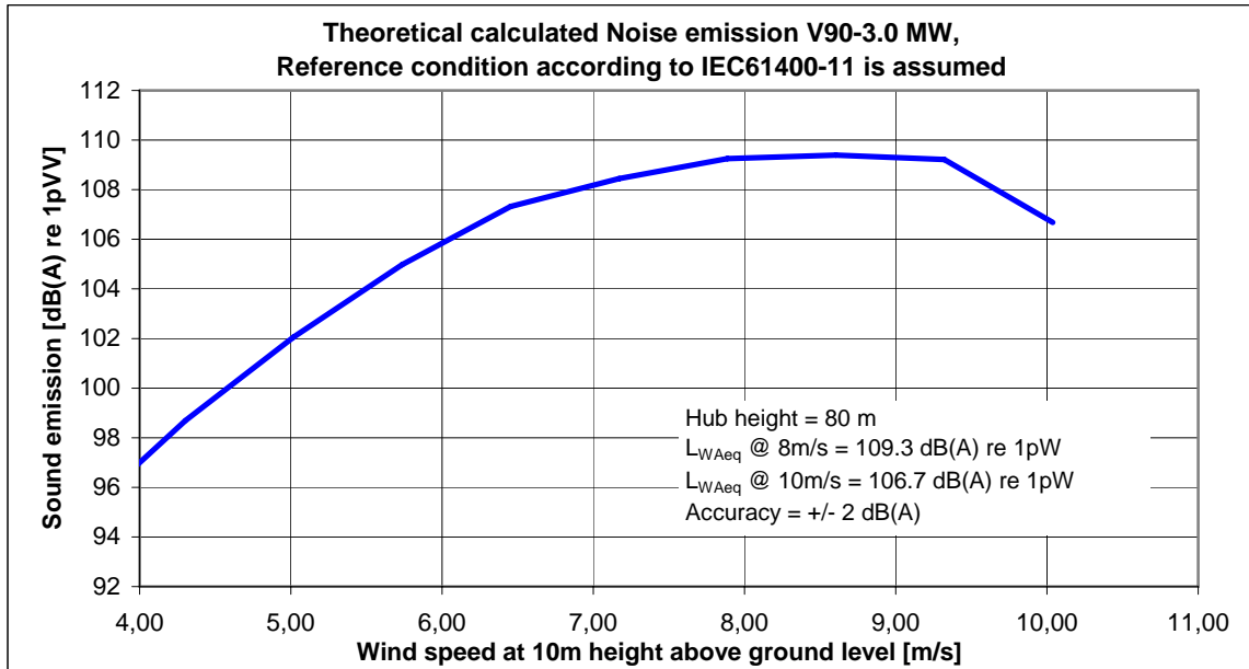
Fig. 7 Noise Emission V90 – 3.0 MW, 60 Hz: Mode 0 measures at 9 m/s in 10 m height
