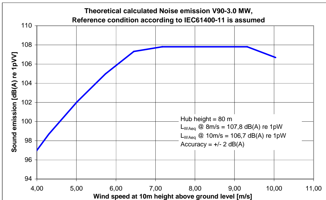
Fig. 8 Noise Emission V90 – 3.0 MW, 60 Hz: Mode 1 measures at 8 m/s in 10 m height
