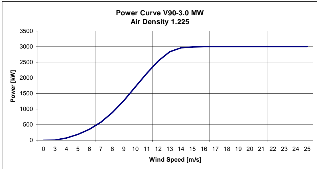
Fig. 2 Power curve for VESTAS V90 – 3.0 MW, 60 Hz Mode 0
