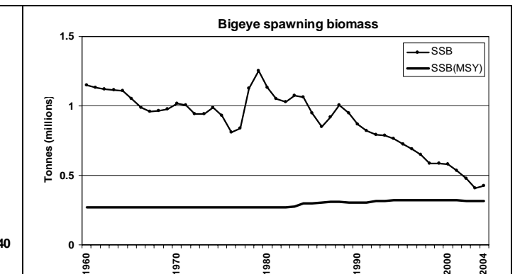
Figure 9. 2006 bigeye tuna stock assessment (ASPM): Spawning stock trajectories relating estimates of annual spawning stock size and the estimated maximum sustainable yield of the spawning stock biomass.
