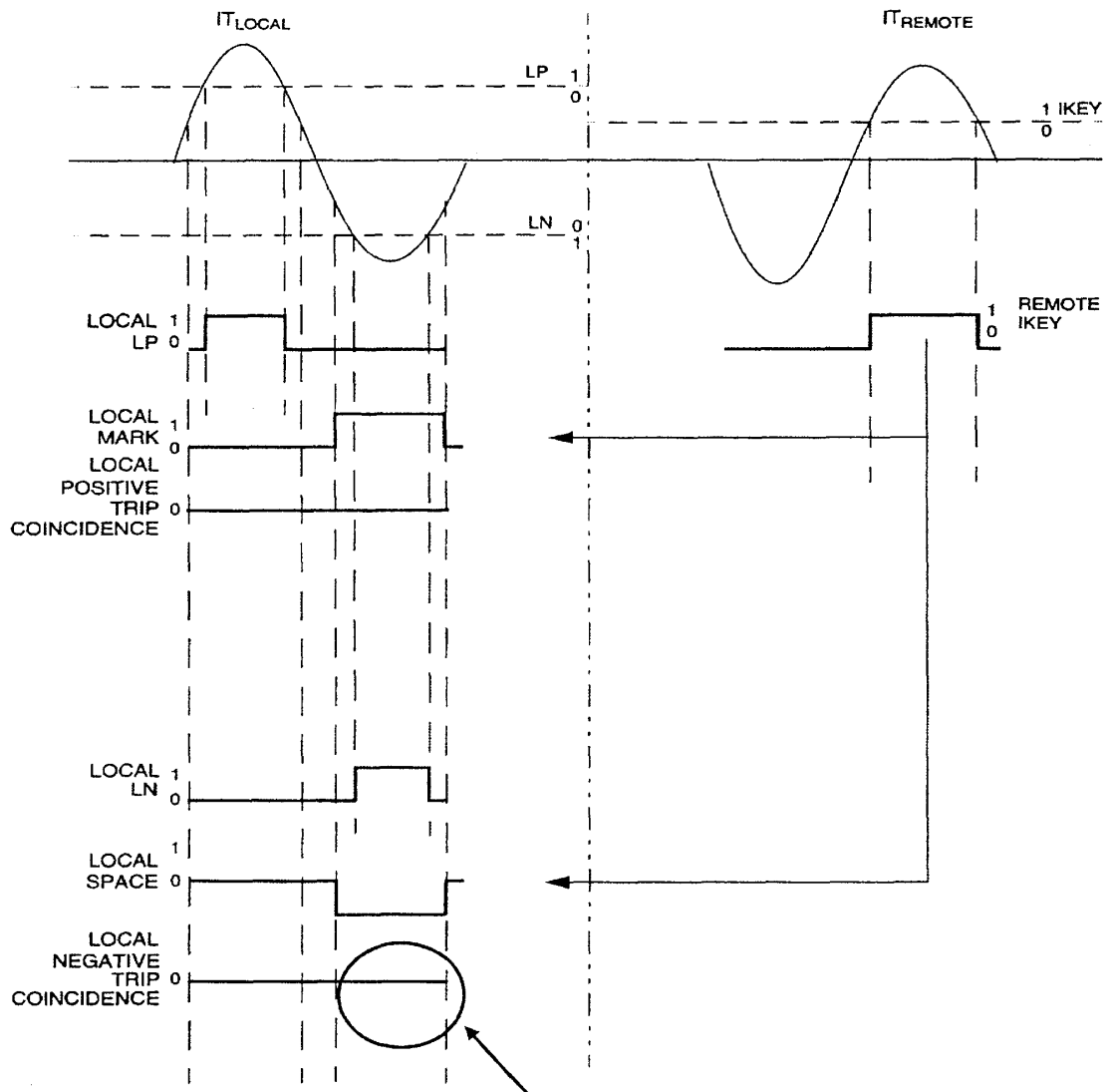
Figure 12b. FSK phase comparison, external fault – no trip
