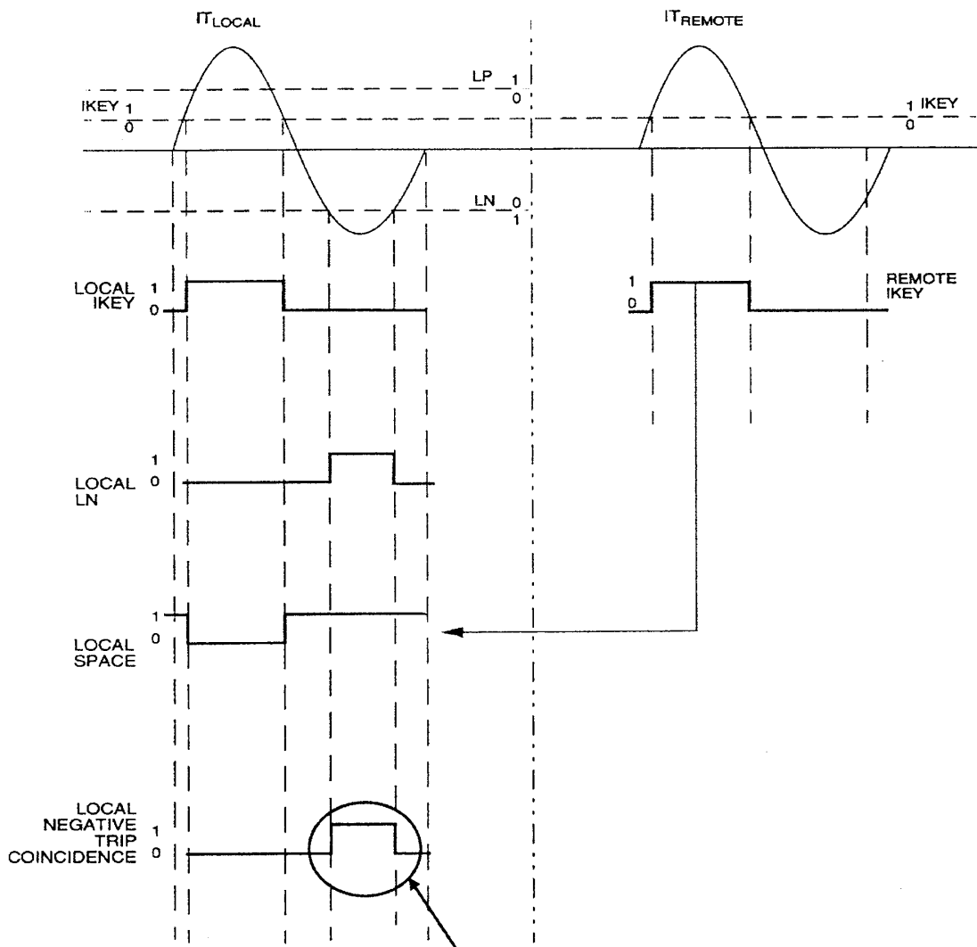
Figure 11a. ON/OFF phase comparison, internal fault - trip
