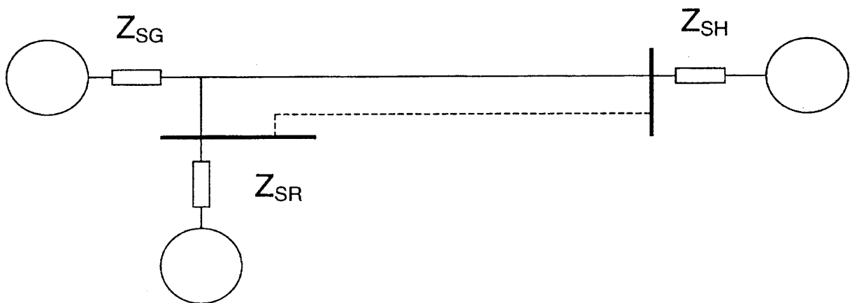
Figure 15. Three terminal application
