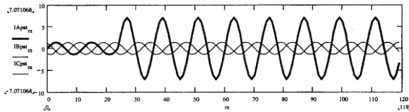
Figure 9a. Fault and load currents
