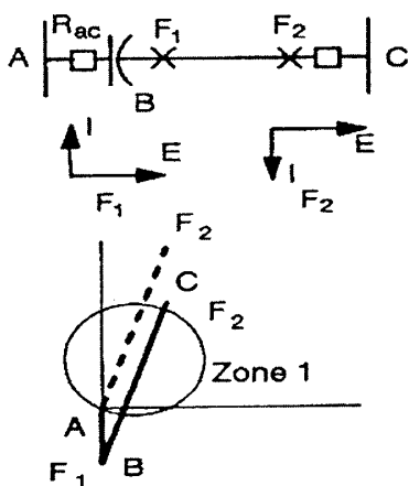
圖一：R-X diagram with a series capacitor.
