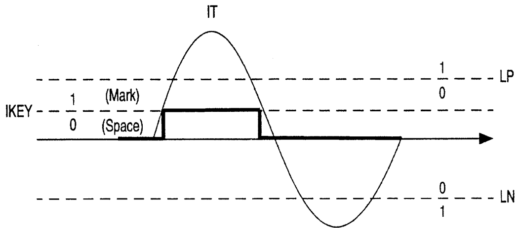
Figure 10. Square wave for keying
