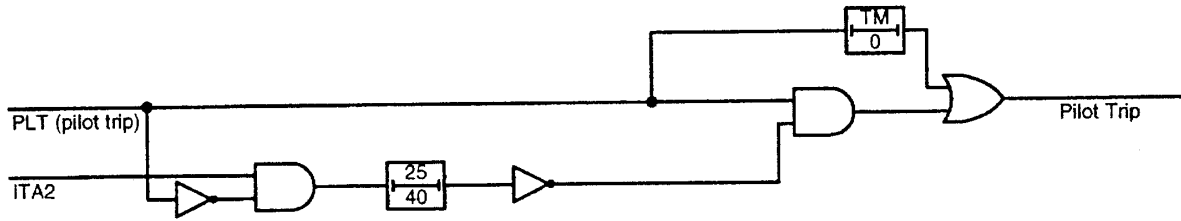
Figure 14. Transient block logic
