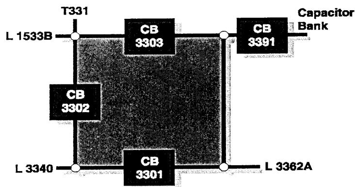
Figure 1. Circuit breaker 3391 (center) and capacitor bank (right).
