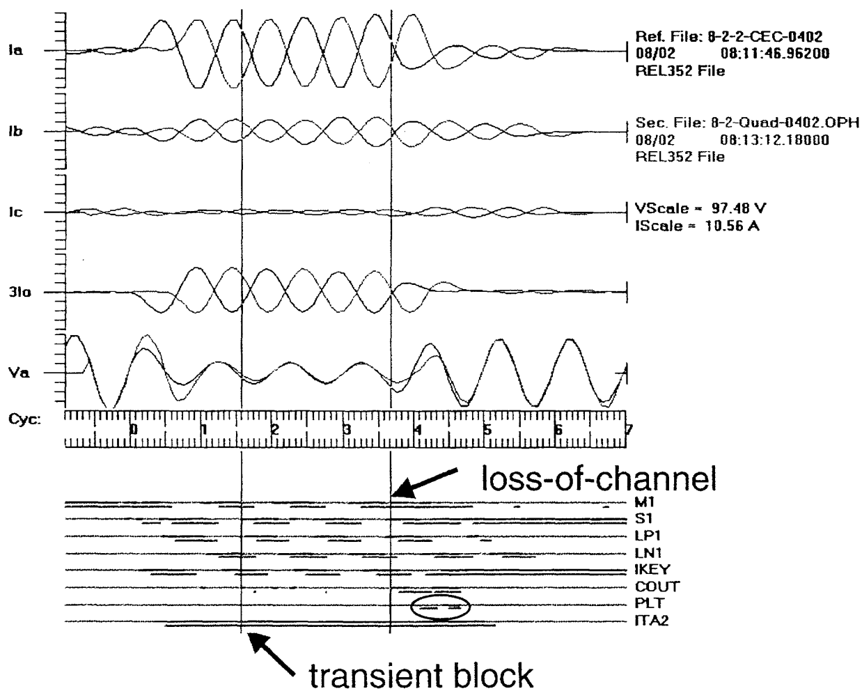
Figure 13. Trip for channel loss at external fault
