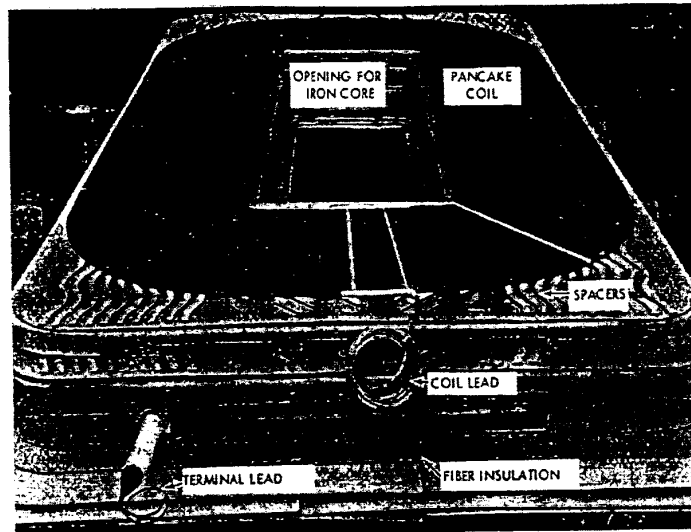
Fig. 3-3. Pancake coil and assembly insulation partially insulated, showing spacers between coils for support of turns.
