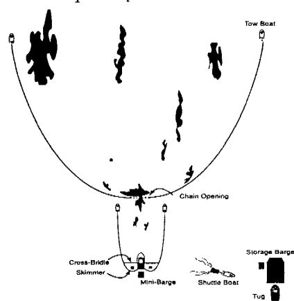
Open Apex U-Boom
