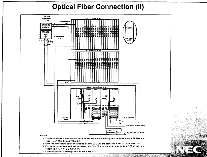
Optical Fiber Connections: Intermediate TERM without DCF
