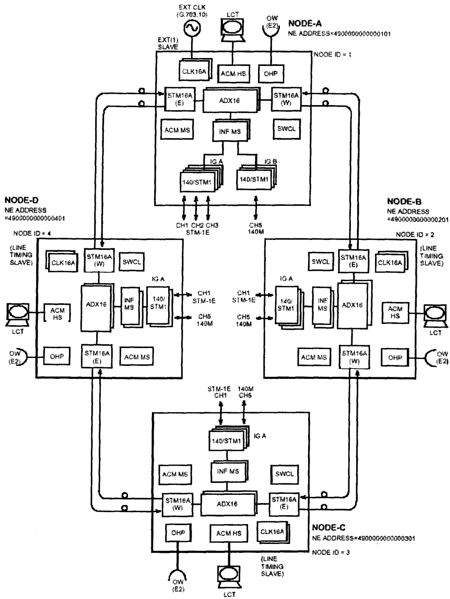
圖九 2F-BLSR MODE MODEL SYSTEM OUTLINE
