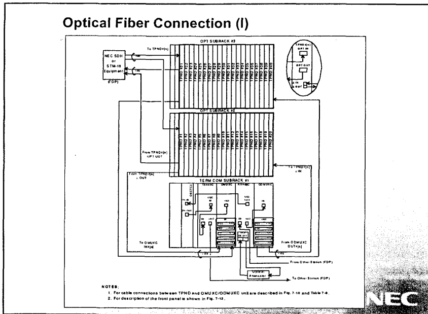
Optical Fiber Connections- End TERM in Full-Open System without DCF
