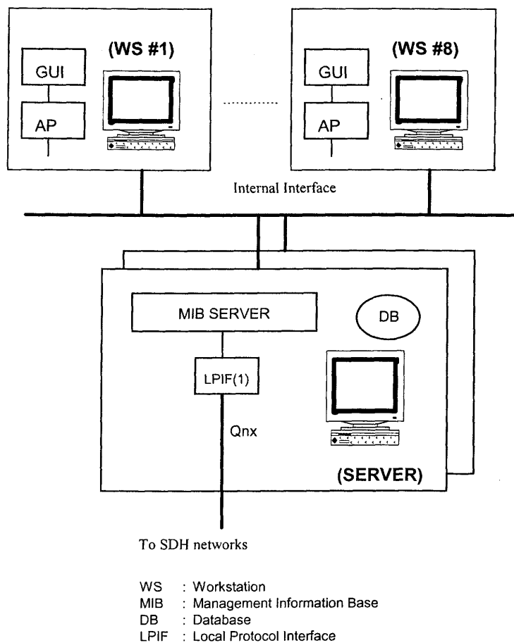
圖一 INC-100MS Architecture
