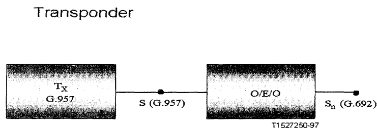
Figure 2/G.692 – Possible implementation of a G.692 transmitter using a G.957 compliant transmitter and a transponder
