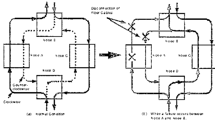
圖5.4.6 SNC-P RING (2F PPS-SHR)
