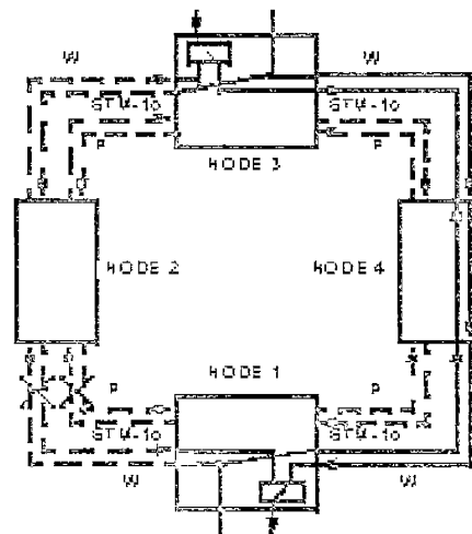
圖5.4.9 SNC-P with Line Protection
