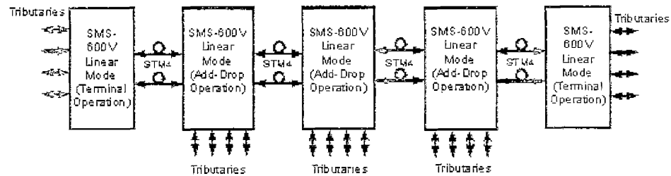
圖5.4.1 Point-to-Point Trunk System應用架構
