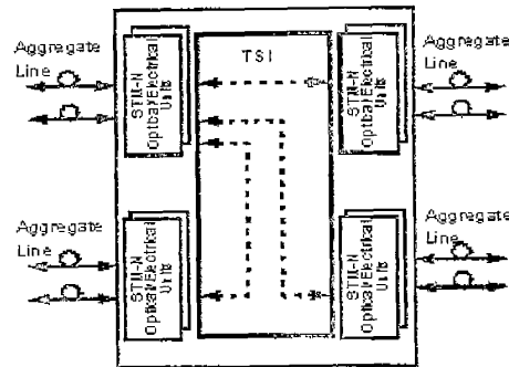
(c) Linear Mode (Local Crossconnect Operation)
