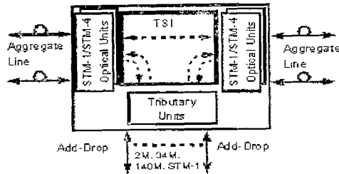
(b) Linear Mode (Add-Drop Operation)
