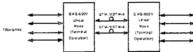
圖5.4.1 Point-to-Point Trunk System應用架構
