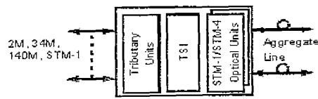
(a) Linear Mode (Terminal Operation)
