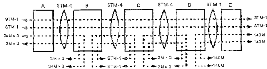
圖5.4.2 Linear Bus with Add-Drop System應用架構圖
