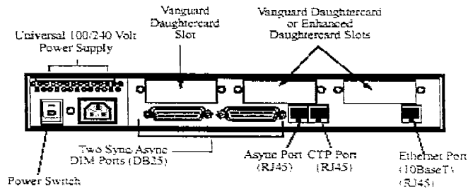
Figure 2-3. Vanguard 6435 Rear Panel
