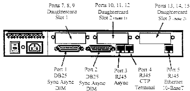
Figure 2-5. Vanguard 6435 Rear Panel Port Numbers
