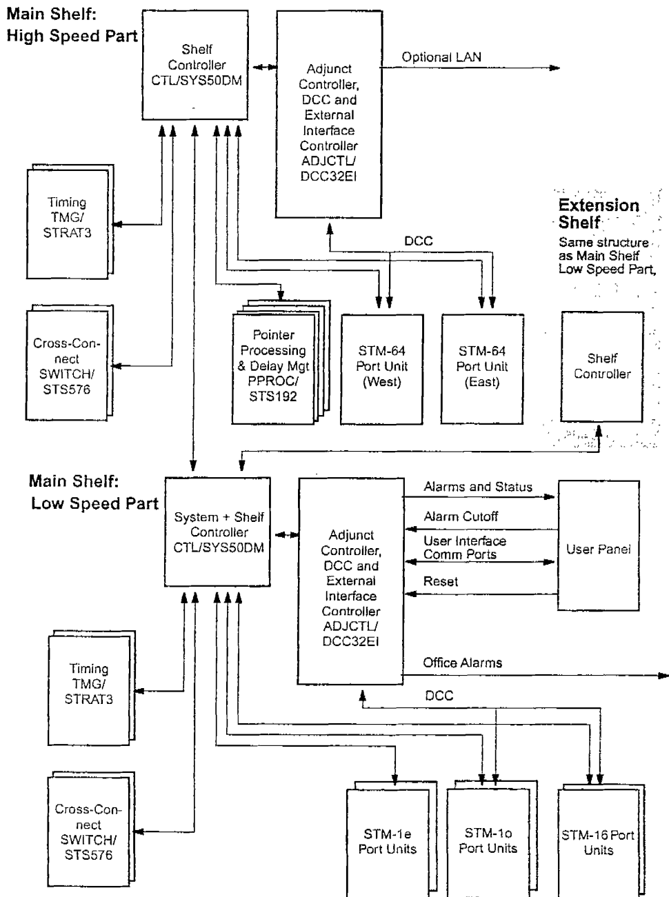
Figure 4-11 WaveStar™ TDM 10G Control Architecture
