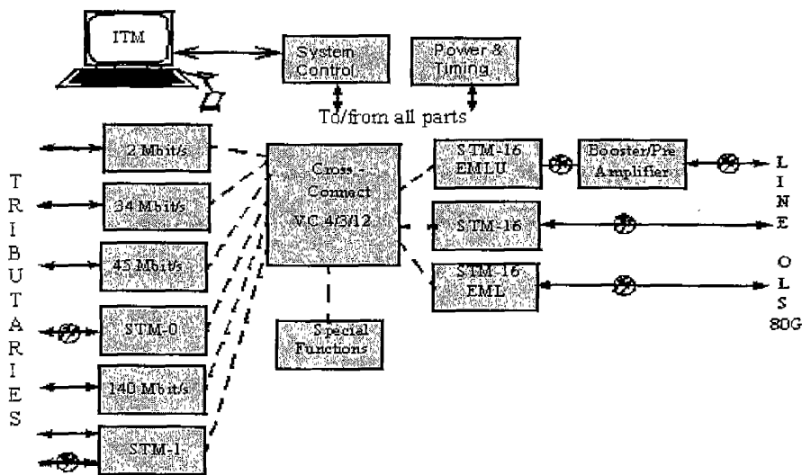
Fig 2-1 Basic WaveStar ADM 16/1 Architecture
