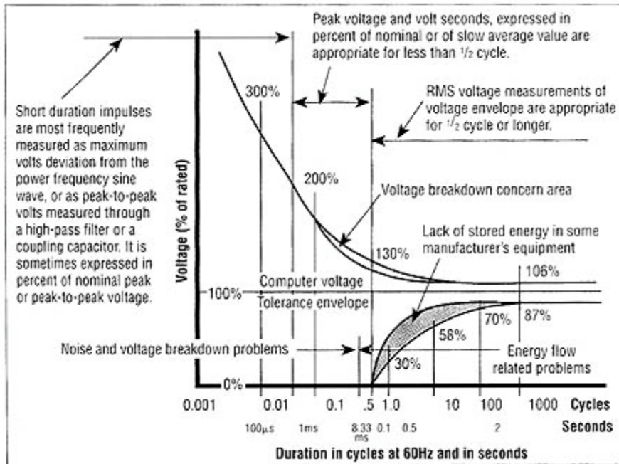
The CBEMA Curve from FIPS No. 94.
