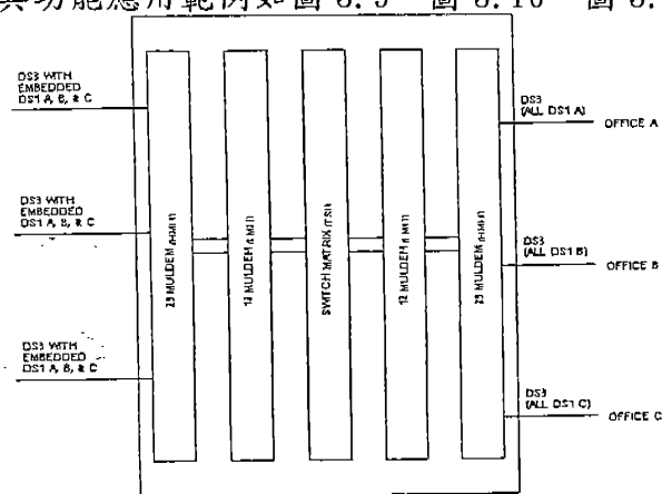
1630 SX Grooming Application Example
