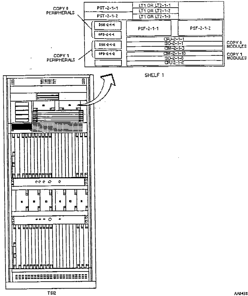
TSI/APM Rack APM Module Addressing
