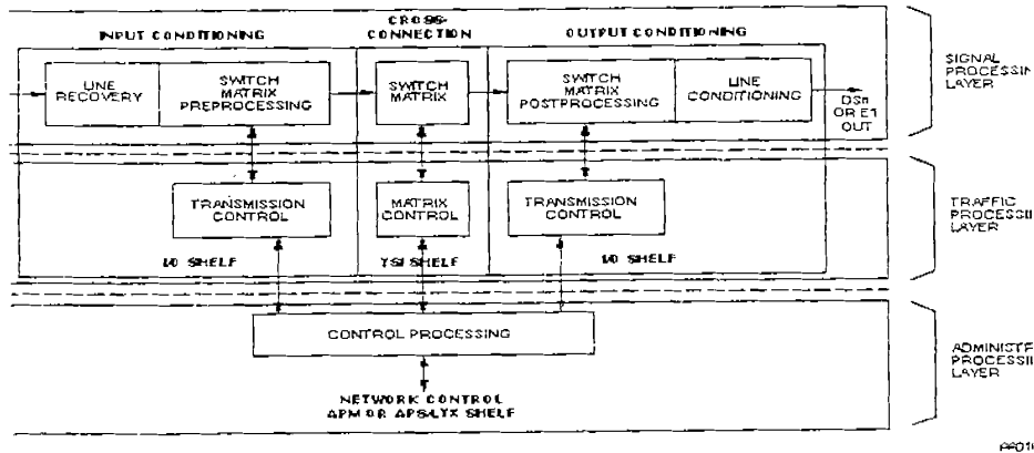
1630 SX Functional Overview for DS1, DS3, and E1 Applications
